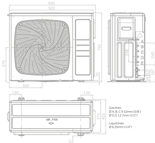
5U90S2SS5FA - 5U105S2SS5FA (5 coupling)
